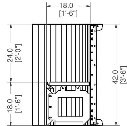
SECTION A-A SCALE 1/12
